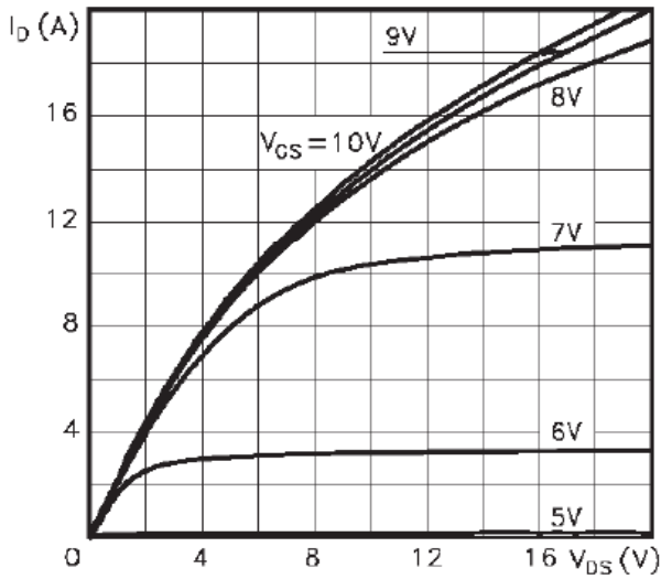
Output Characteristic
