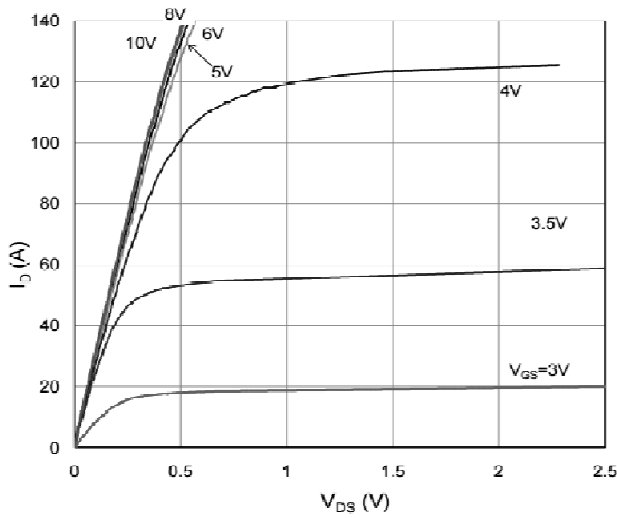
Output Characteristic
