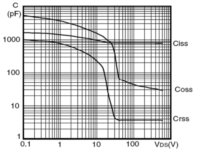
Capacitance
