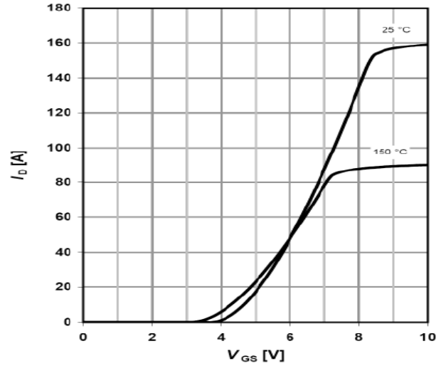
Transfer Characteristic
