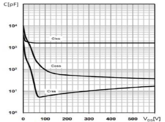
Capacitance
